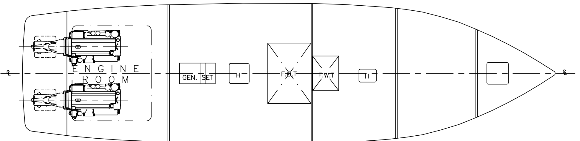
BELOW DECK
