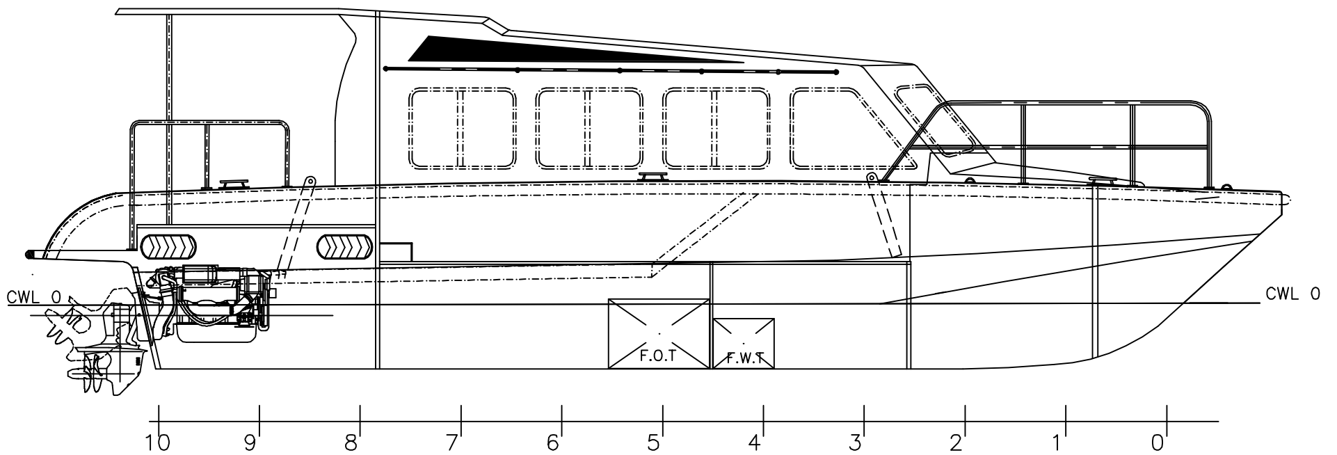
INBOARD PROFILE
