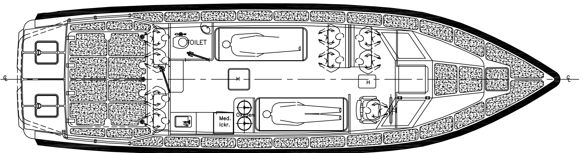
MAIN DECK
