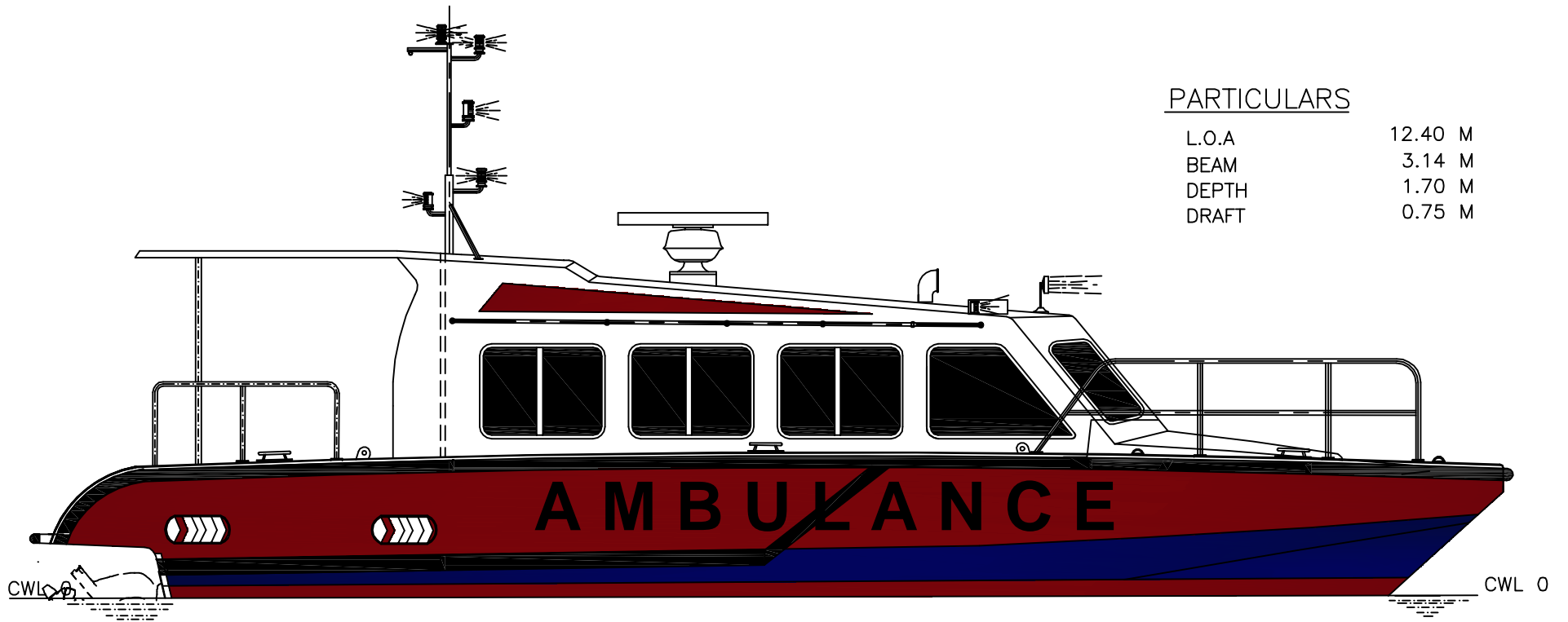
OUTBOARD PROFILE
