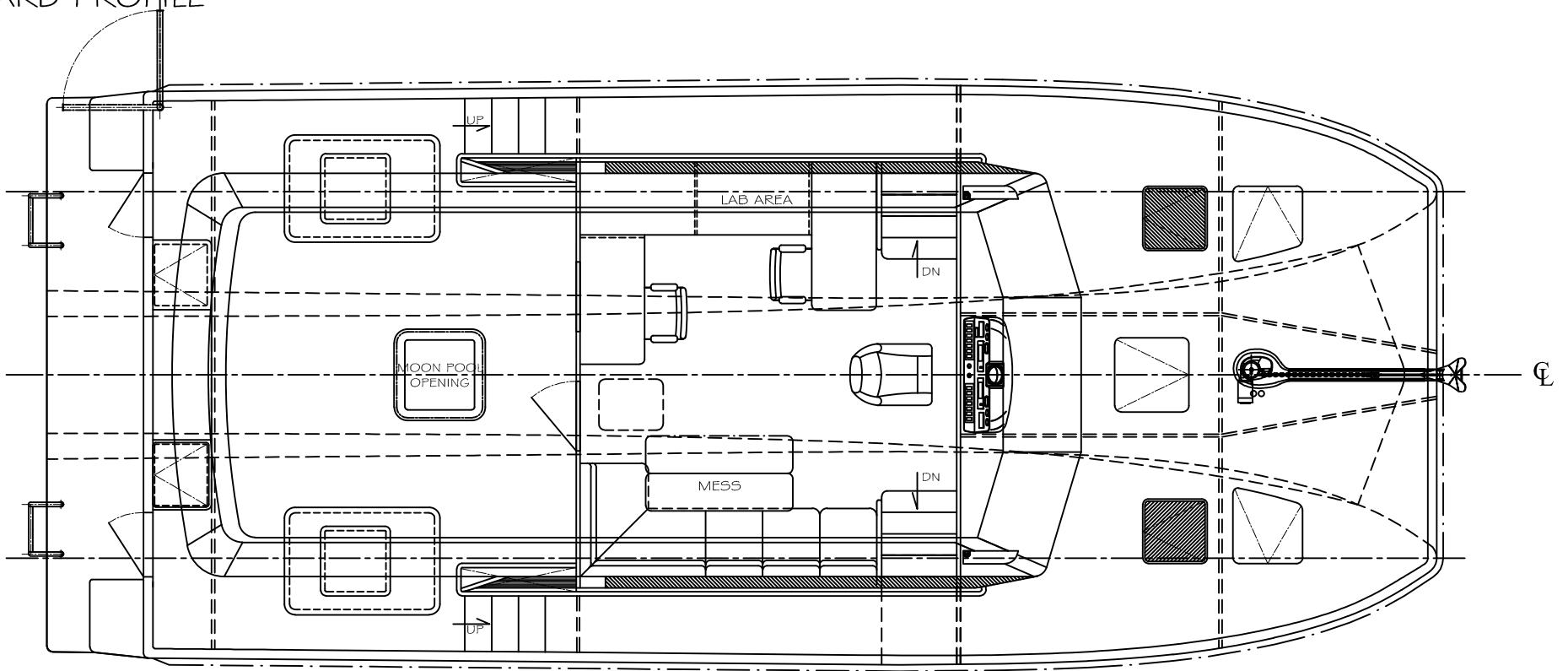
MAIN DECK PLAN
