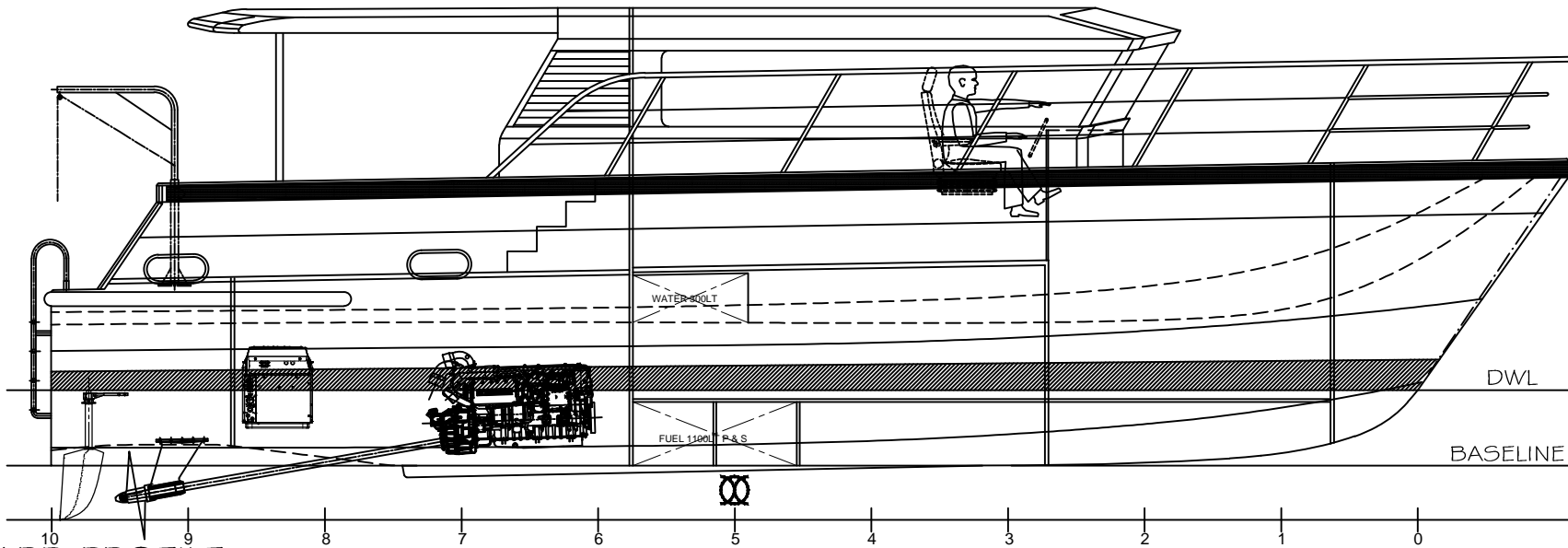
INBOARD PROFILE
