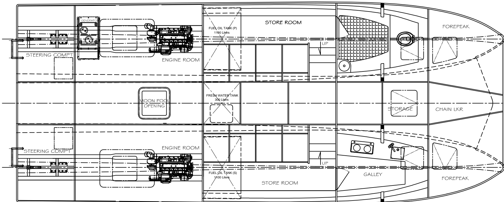
BELOW DECK PLAN
