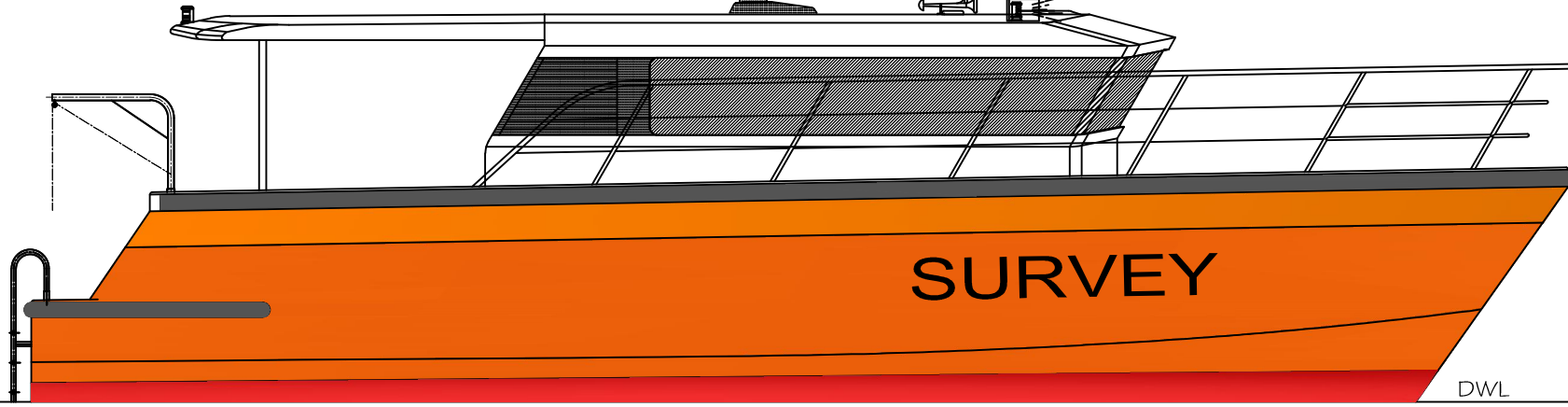
OUTBOARD PROFILE
