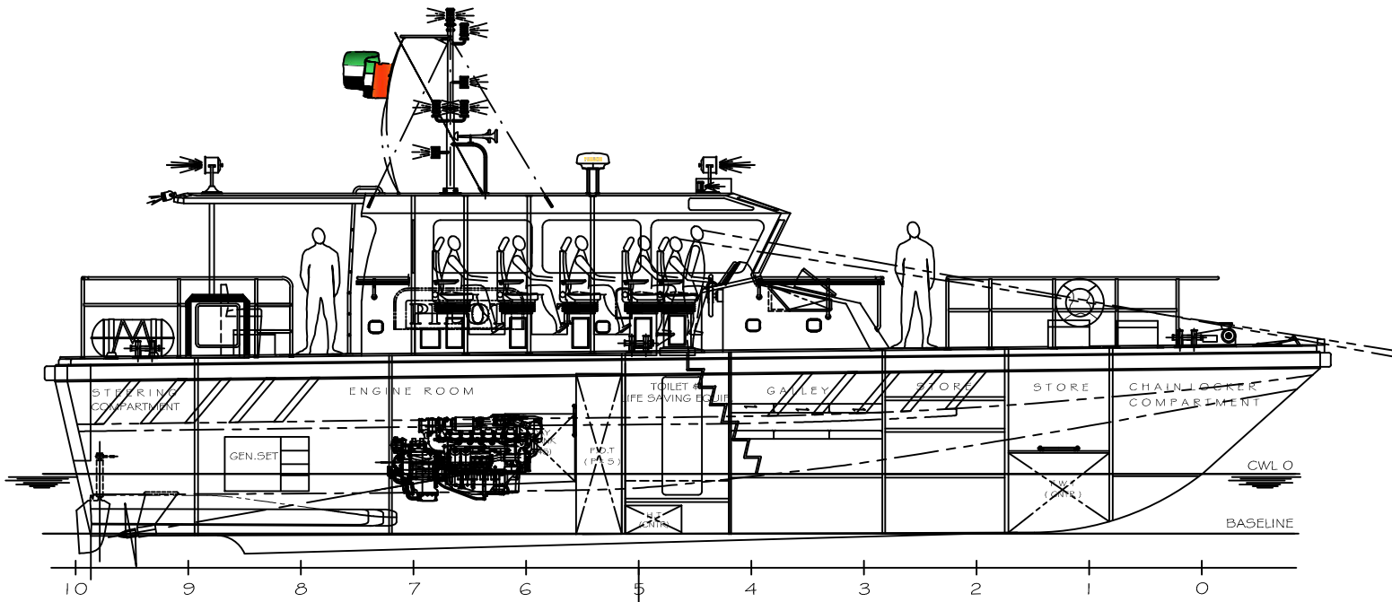
INBOARD PROFILE
