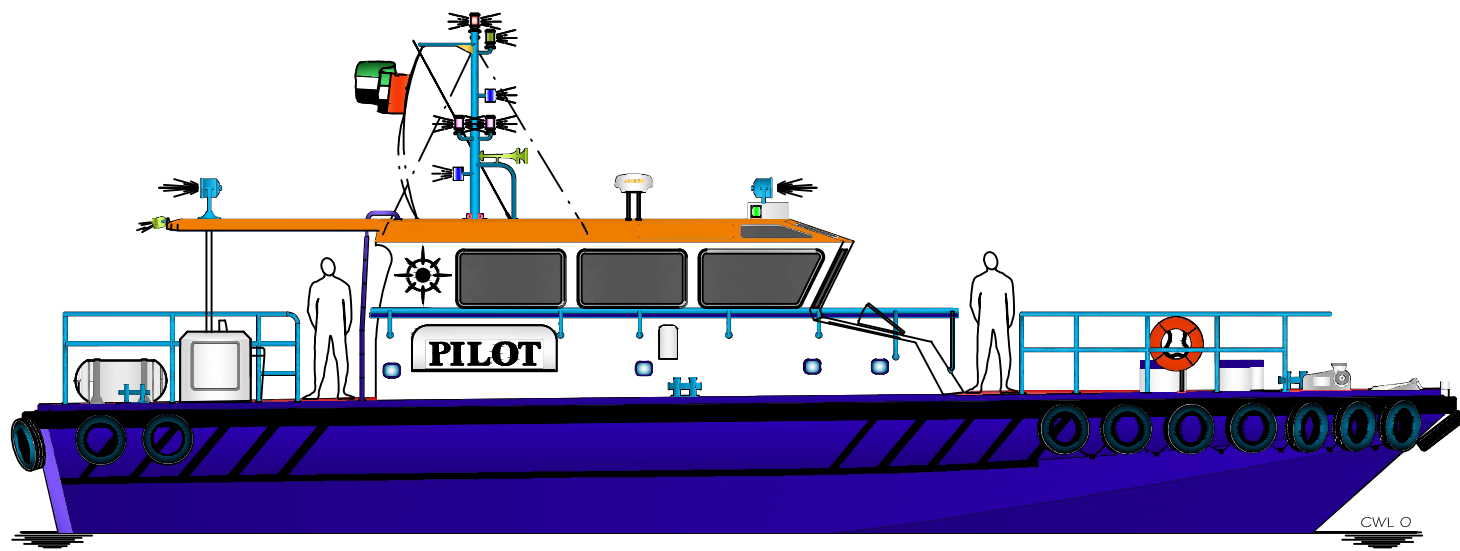
OUTBOARD PROFILE
