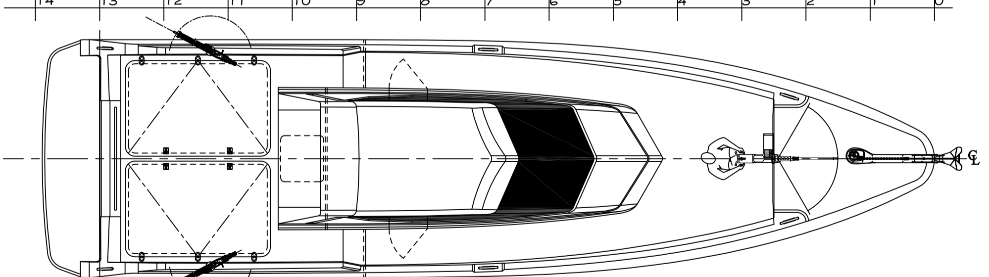
MAIN DECK PLAN
