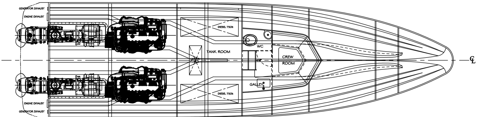
LOWER DECK PLAN
