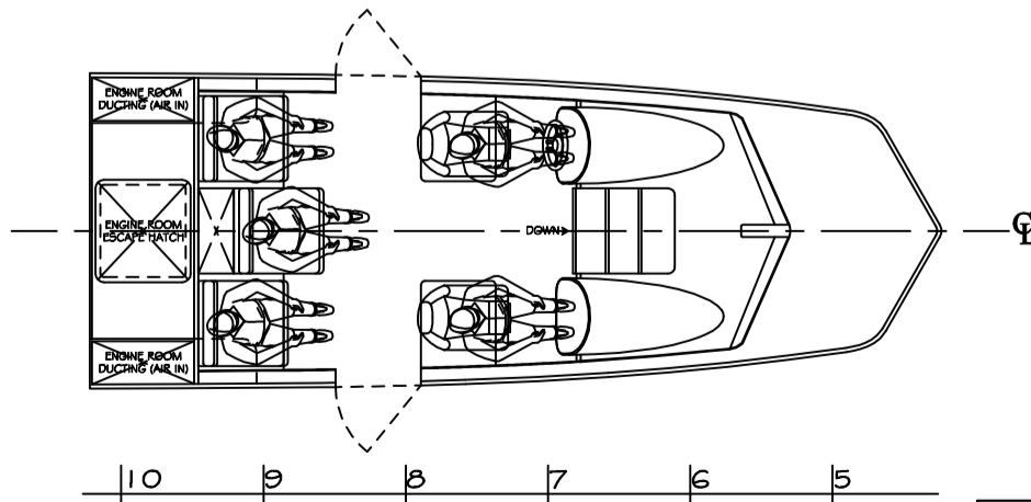
WHEELHOUSE
