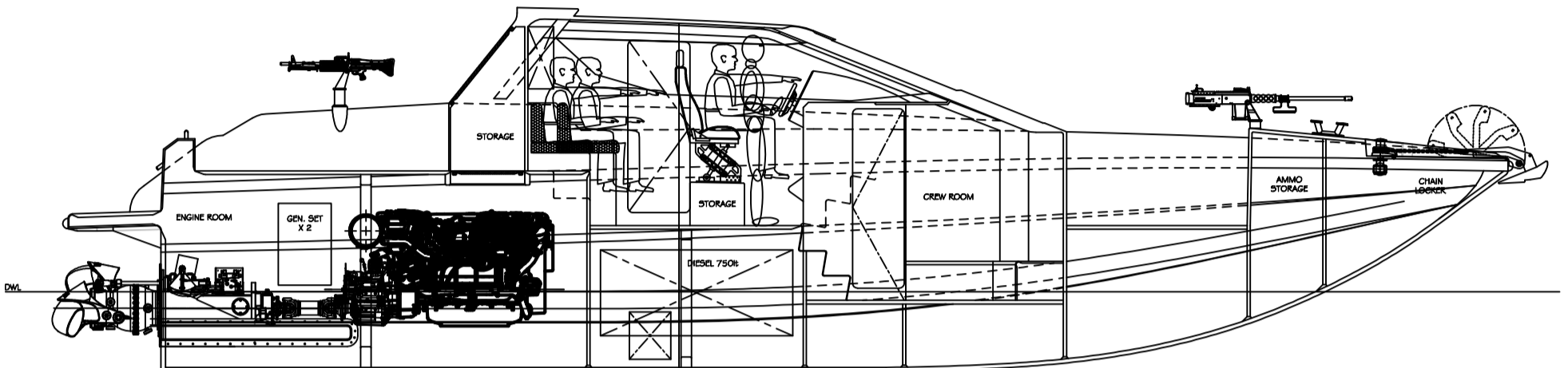
INBOARD PROFILE
