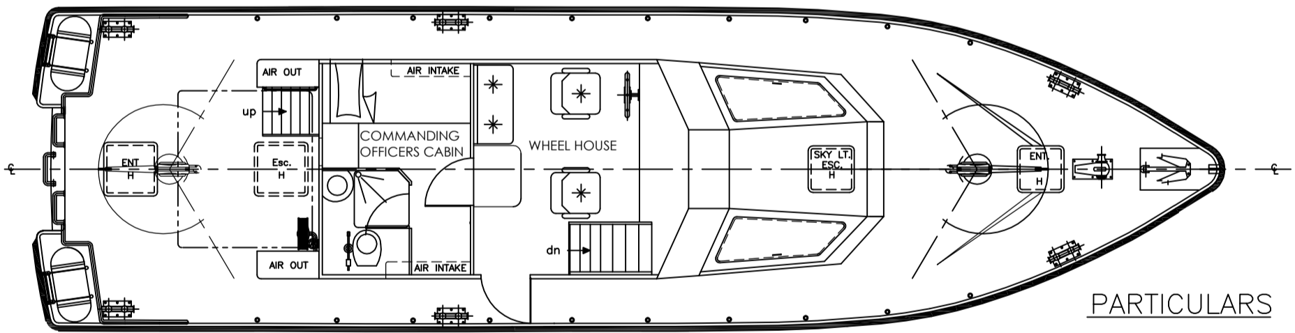
MAIN DECK
