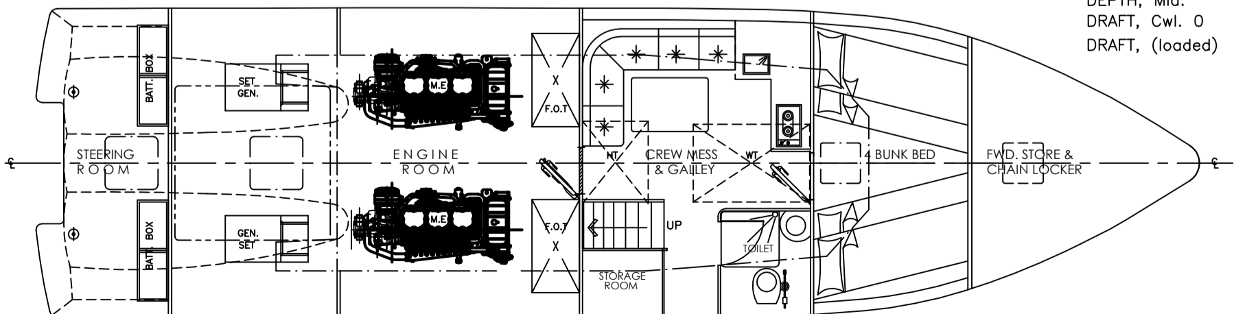
BELOW DECK
