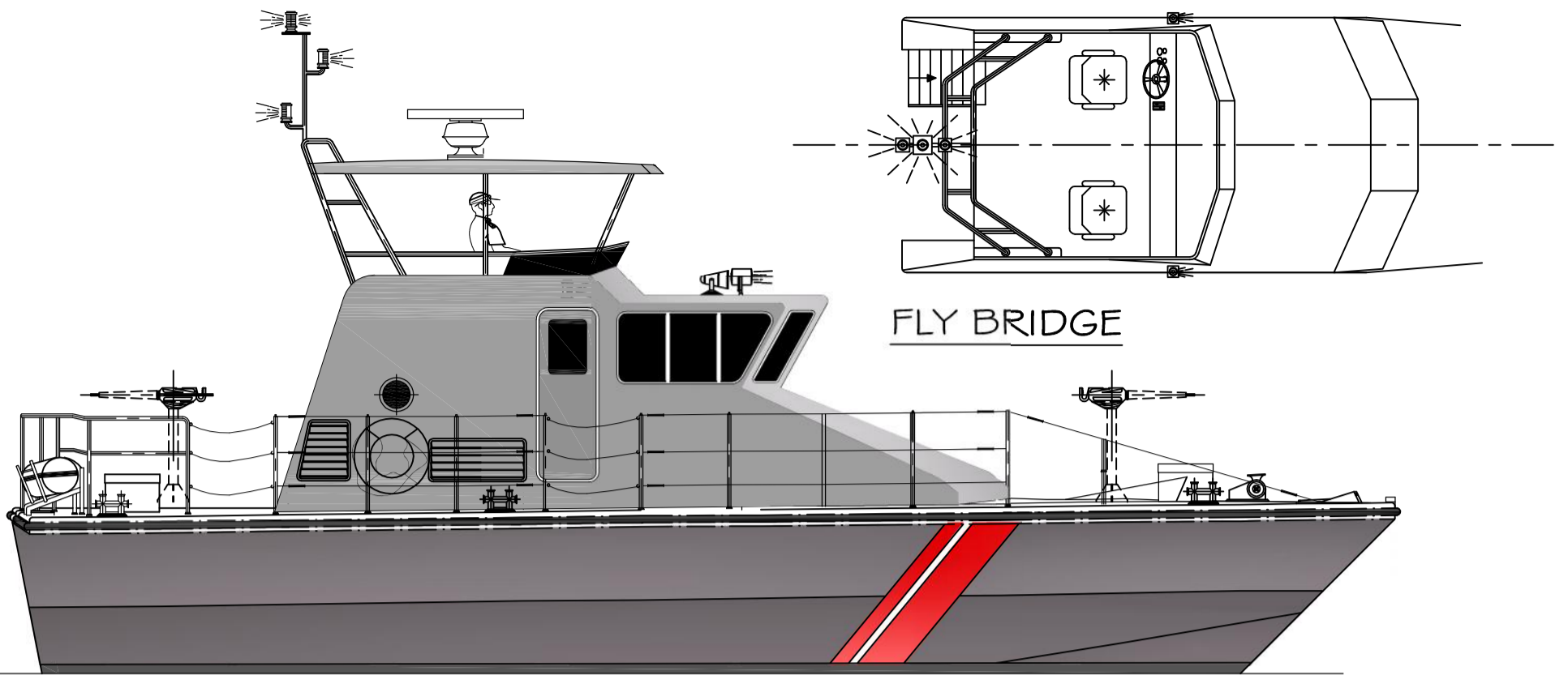
OUTBOARD PROFILE
