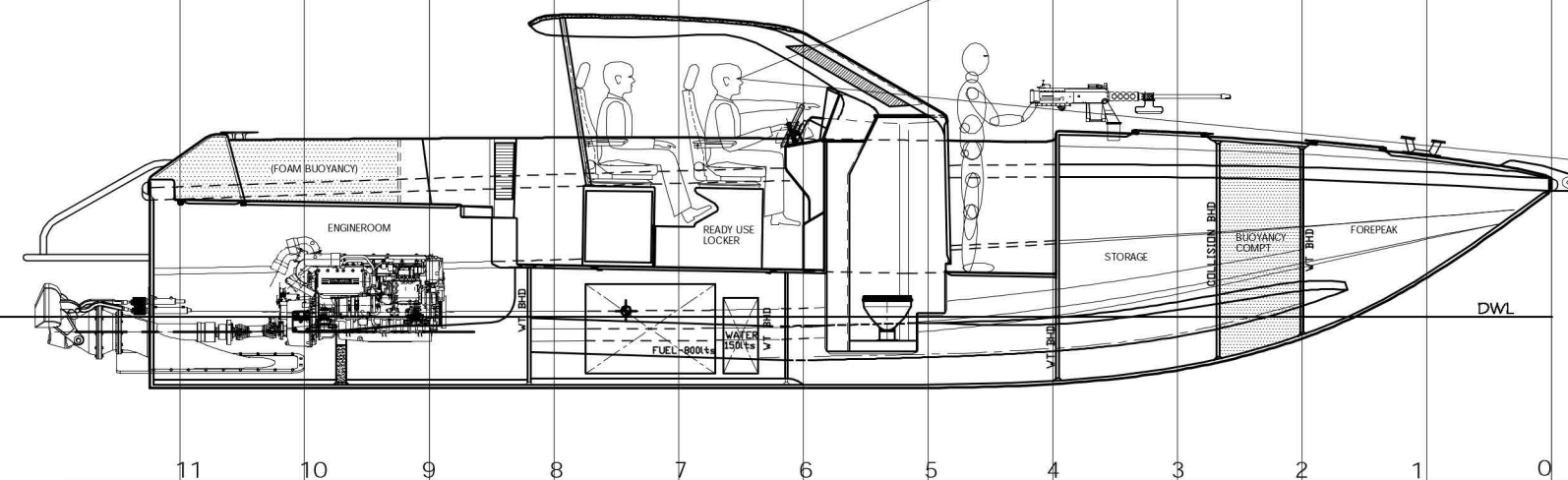
INBOARD PROFILE
