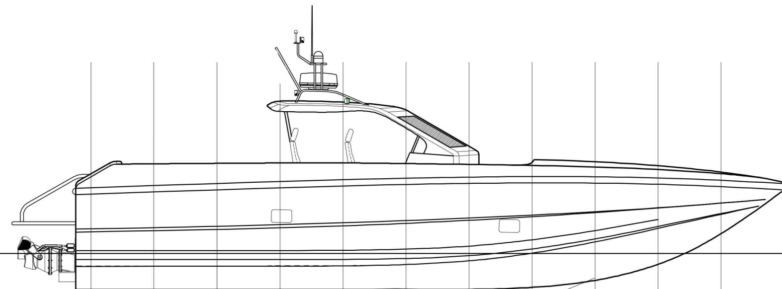
OUTBOARD PROFILE
