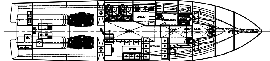
BELOW DECK
