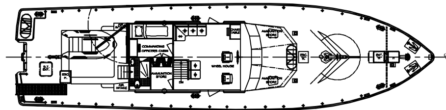
MAIN DECK
