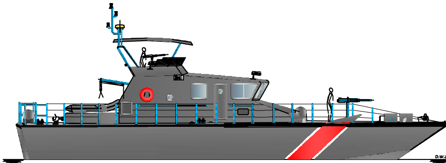
OUTBOARD PROFILE
