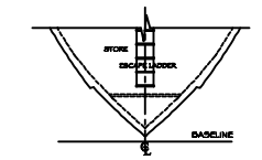
STATION 1 VIEWING TO FORE
