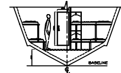
STATION 3 VIEWING TO AFT
