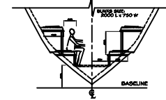
STATION 1.5 VIEWING TO AFT
