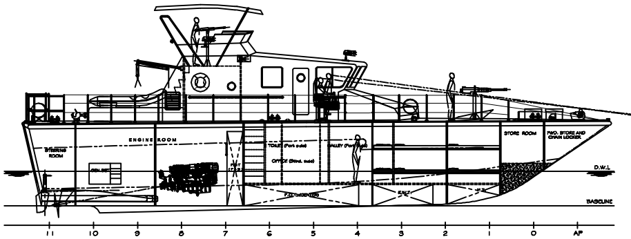
INBOARD PROFILE
