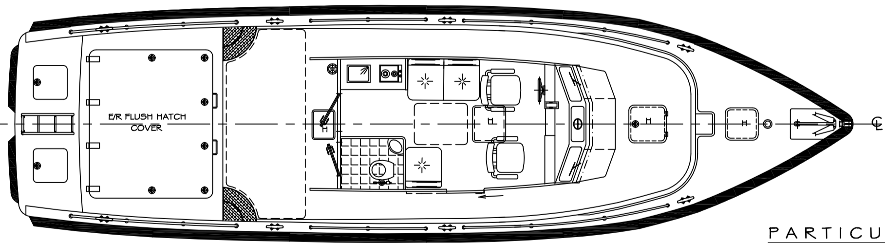
MAIN DECK
