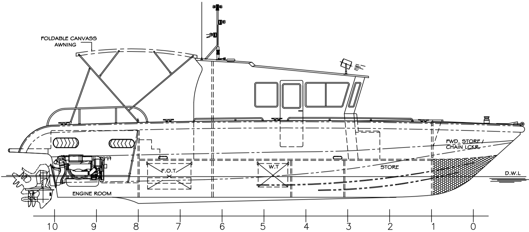
INBOARD PROFILE
