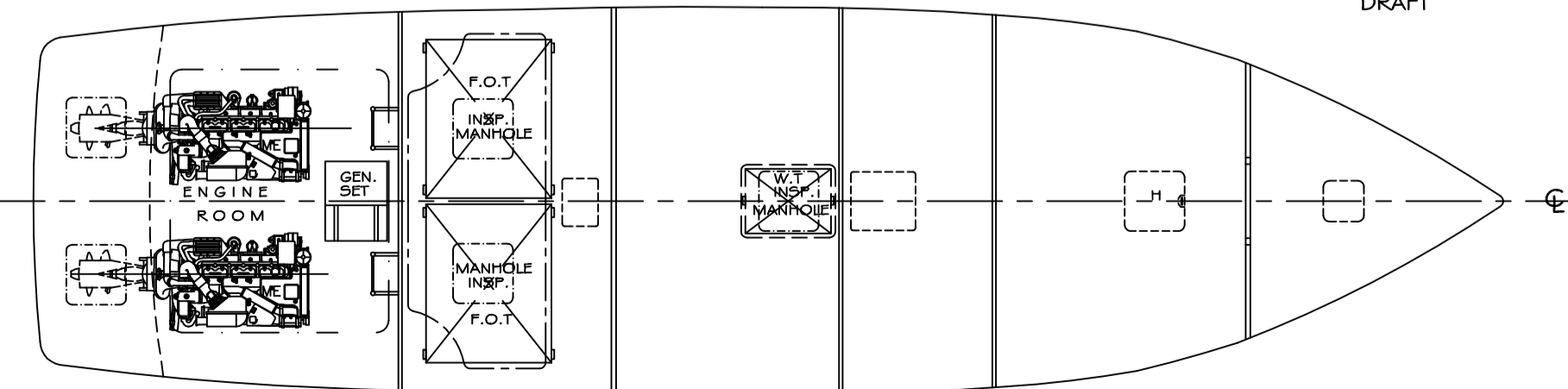
BELOW DECK
