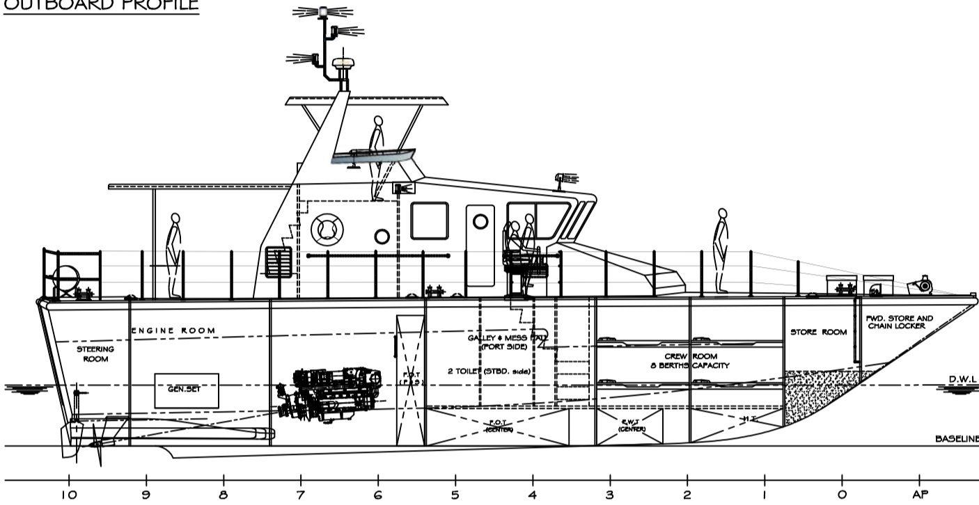
INBOARD PROFILE
