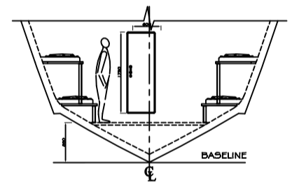
STATION 3 VIEWING TO AFT
