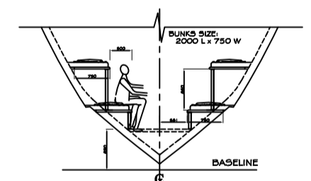
STATION 1.5 VIEWING TO AFT
