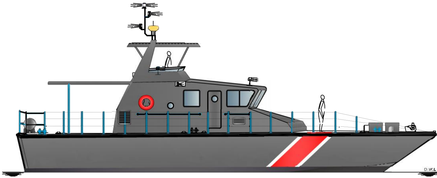
OUTBOARD PROFILE
