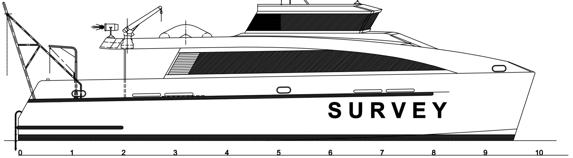
OUTBOARD PROFILE
