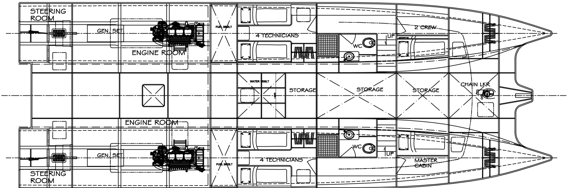
LOWER DECK PLAN
