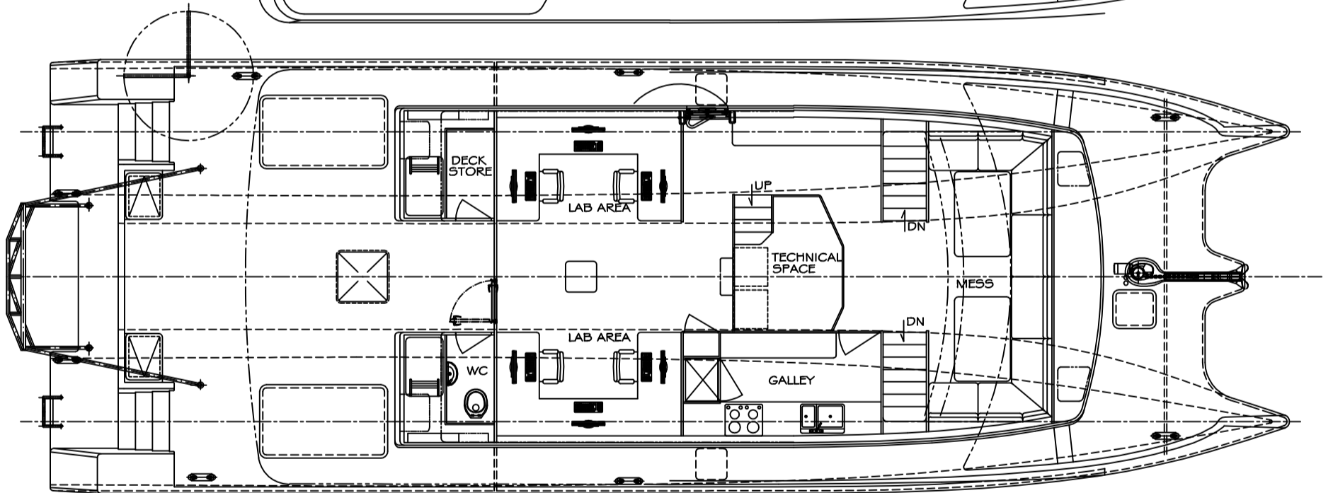
MAIN DECK PLAN
