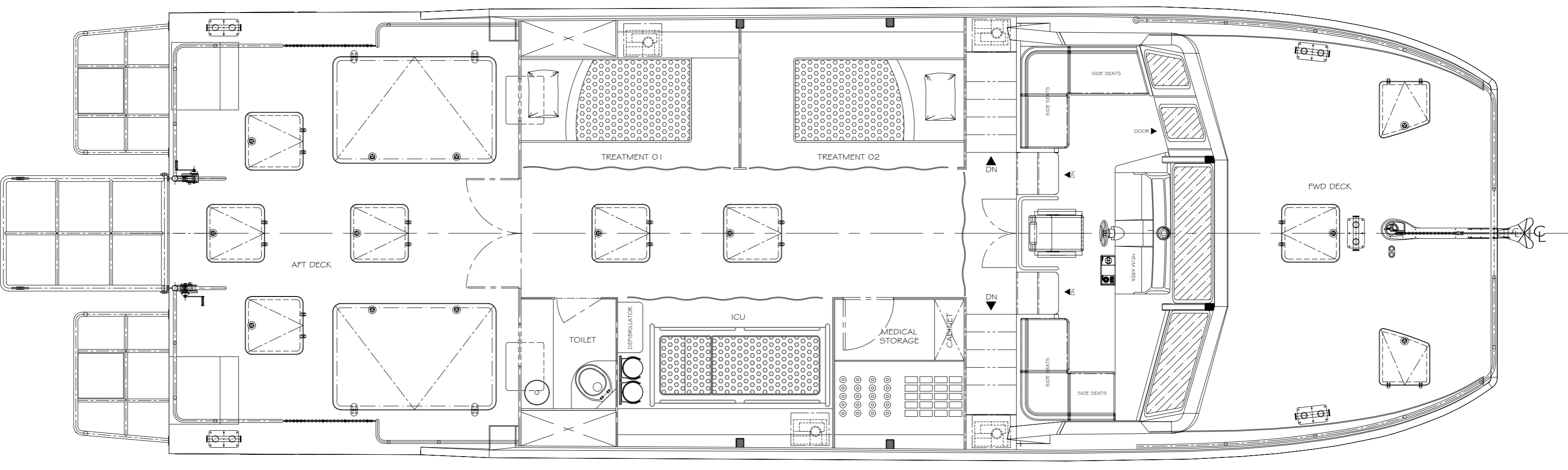
MAINDECK (INTERIOR ARRANGEMENT)
