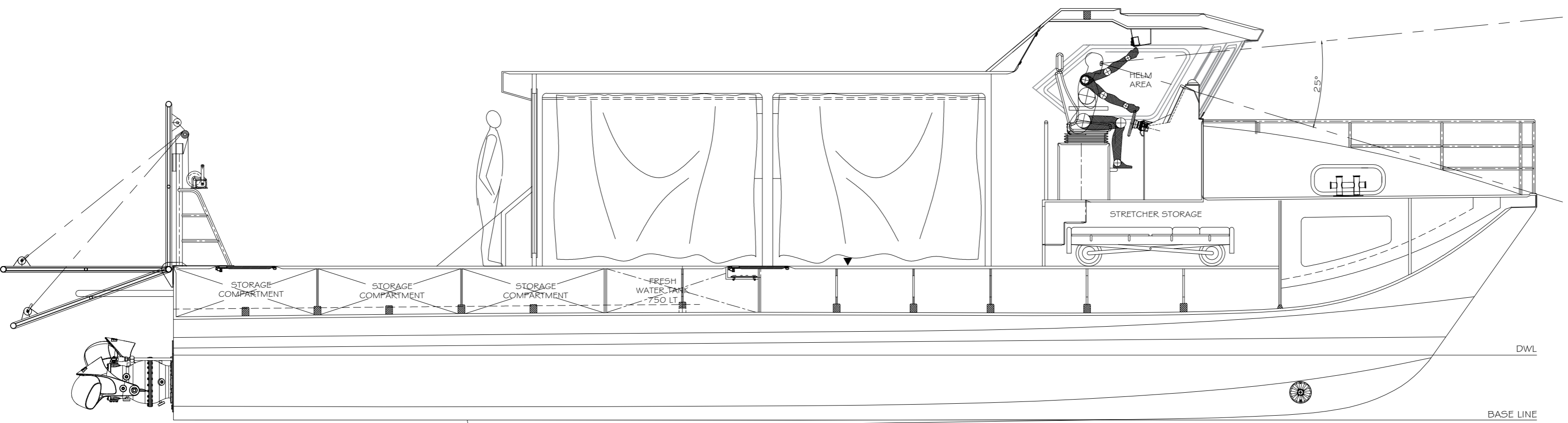
VESSEL CENTER LINE SECTION
