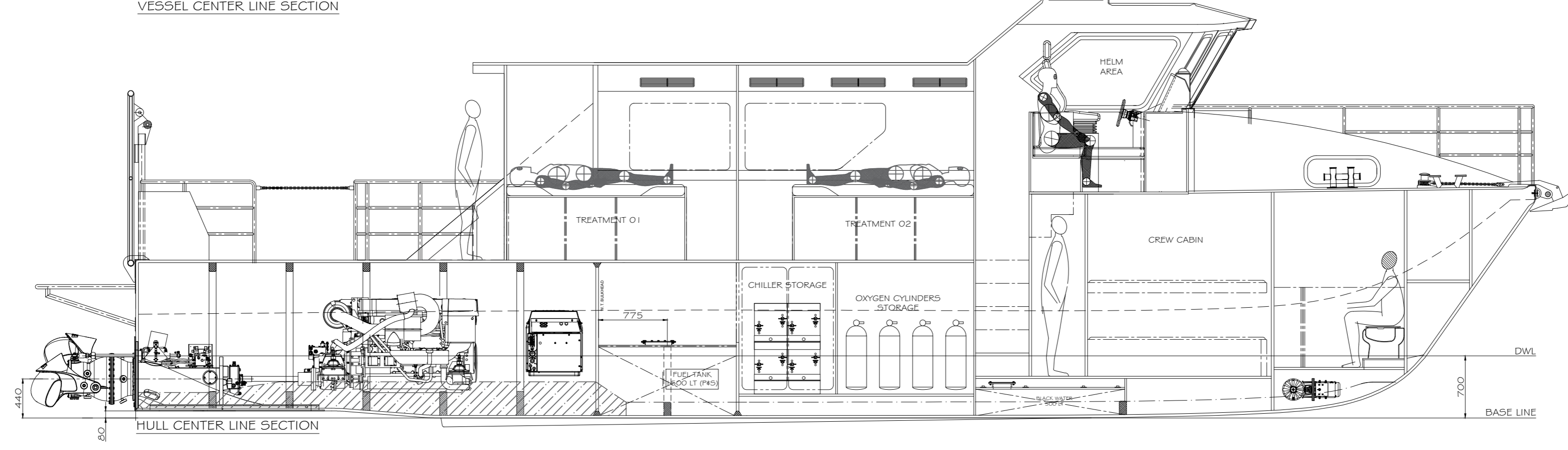
HULL CENTER LINE SECTION
