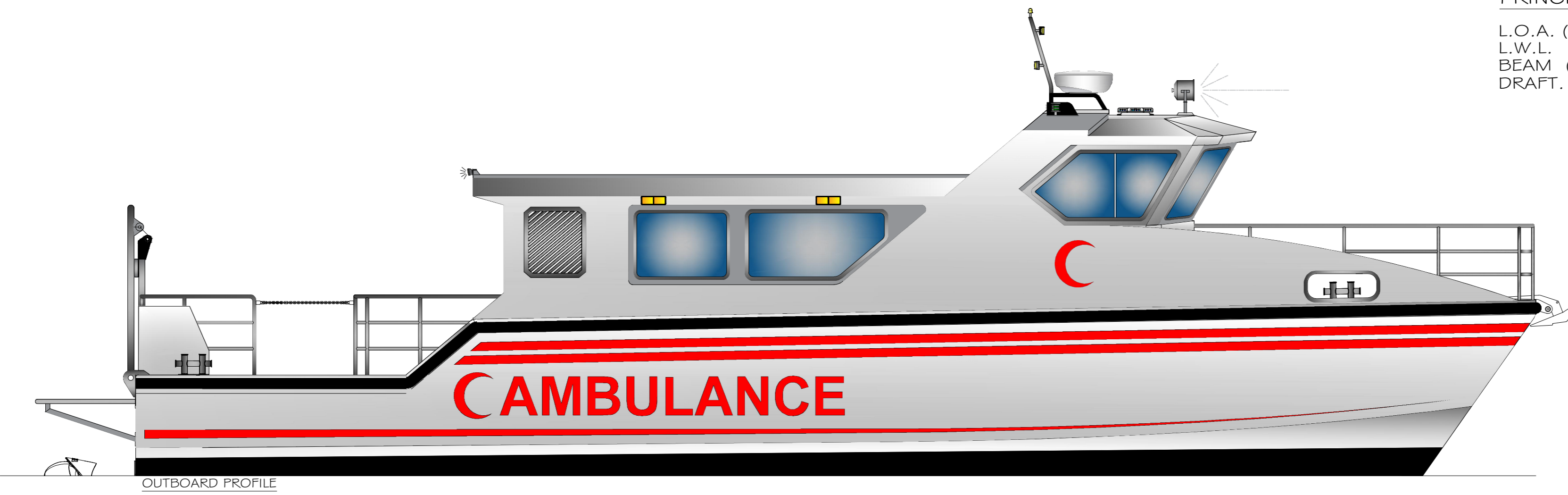
OUTBOARD PROFILE
