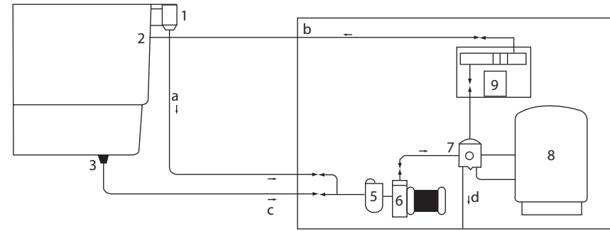
Filtration Plant
