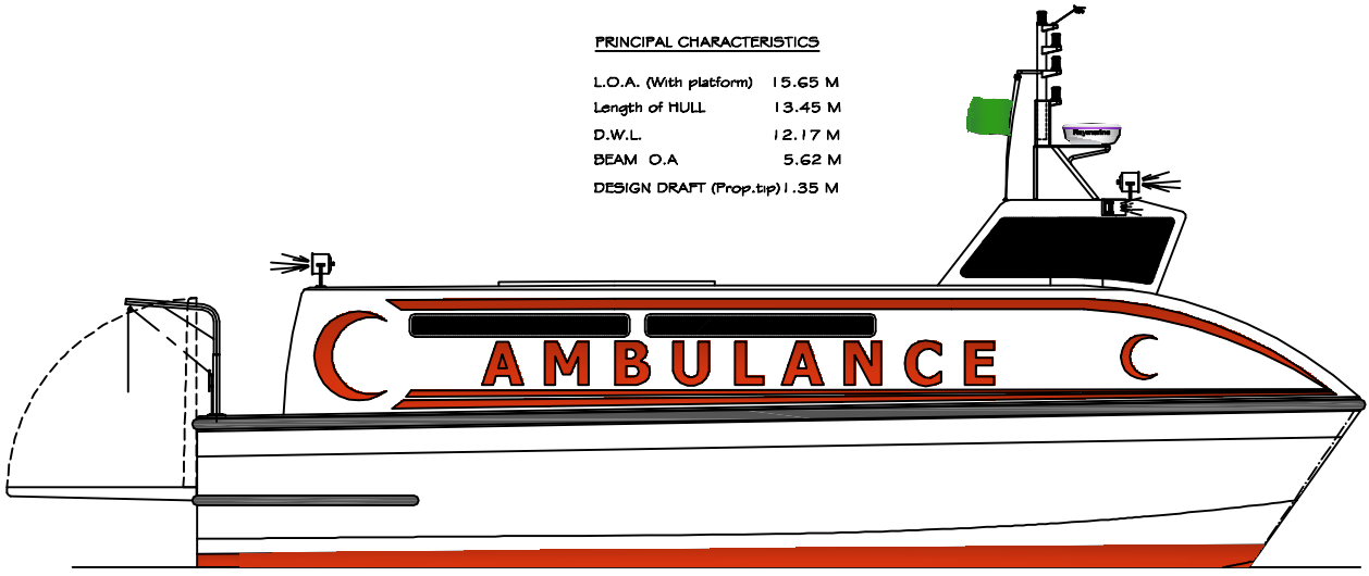
OUTBOARD PROFILE
