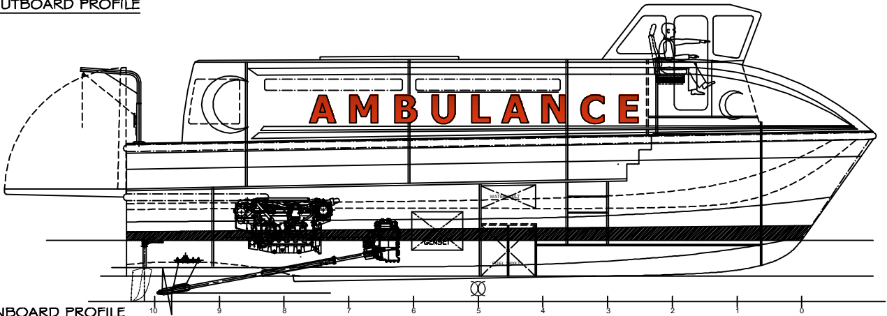
INBOARD PROFILE
