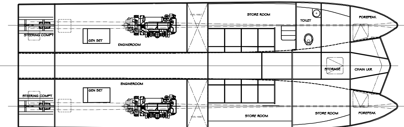
BELOW DECK PLAN
